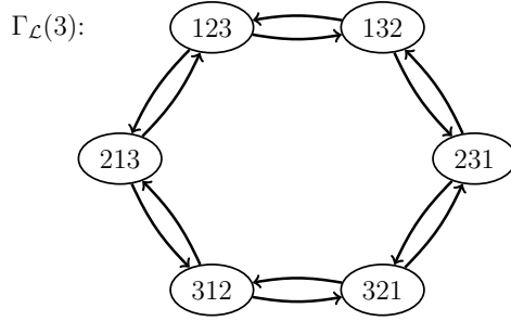
Figure 2: The digraph \Gamma_{\mathcal{L}}(3)
