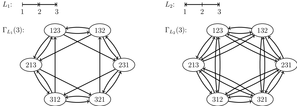
Figure 1: The digraphs \Gamma_D(3) for D = L_1 and D = L_2
