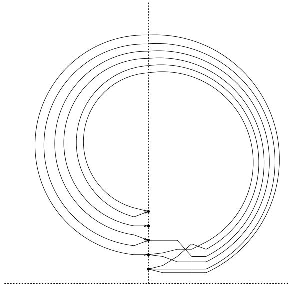
Figure 2: \text{CR}^*(G) \leq e - 1 .
