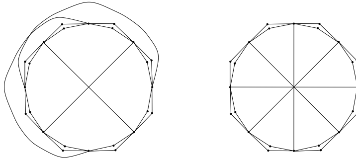
Figure 1: \text{CR}(G) = 2, \text{CR}^*(G) = 1 .
