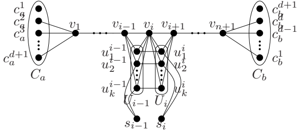
Figure 1: A construction used in Theorem 4.2
