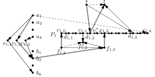
Figure 2: The gadget used in the reduction to DIRECTED DISJOINT PATHS. Only the path P_1 is shown. The dashed arrows show some of the demands in the gadget, the shaded edges give a solution for these demands.
