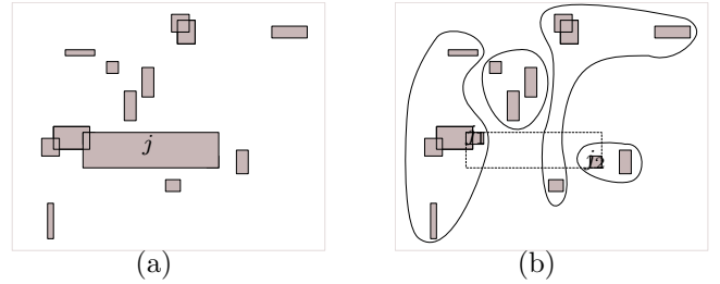
Figure 3: Step i + 1 of the decomposition merges j_1 and j_2 to j . (a) A connected set K of G_{i+1} containing j . (b) Replacing j with j_1 and j_2 gives a set K^{\text{II}} inducing 4 connected components in G_i .
