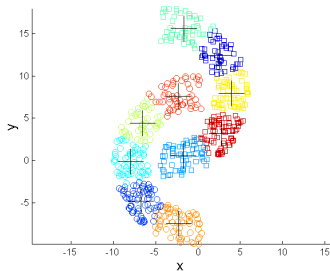
K-means Clusters
